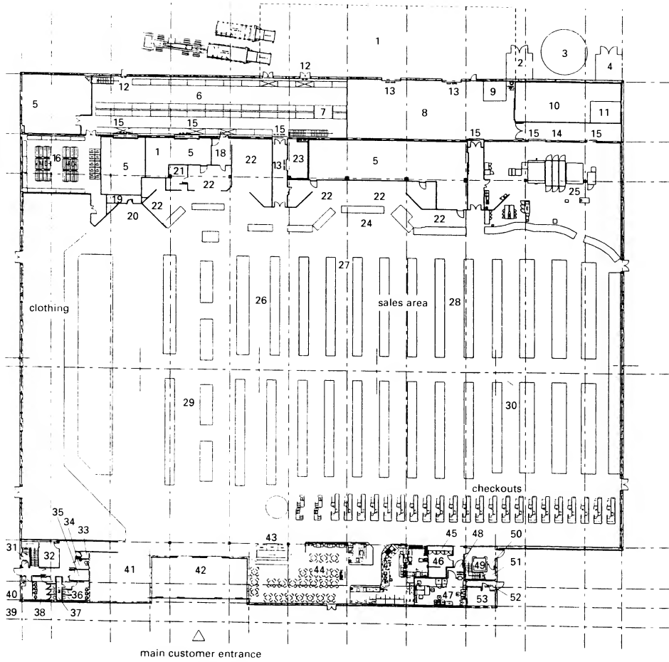
① Floor plan of an Asda supermarket/hypermarket in the UK (courtesy of Asda/WCEC Architects)
